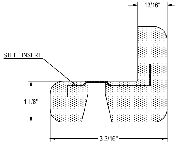
CROSS SECTION
