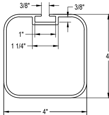
EXTRUSION
