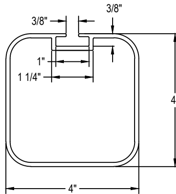
EXTRUSION
